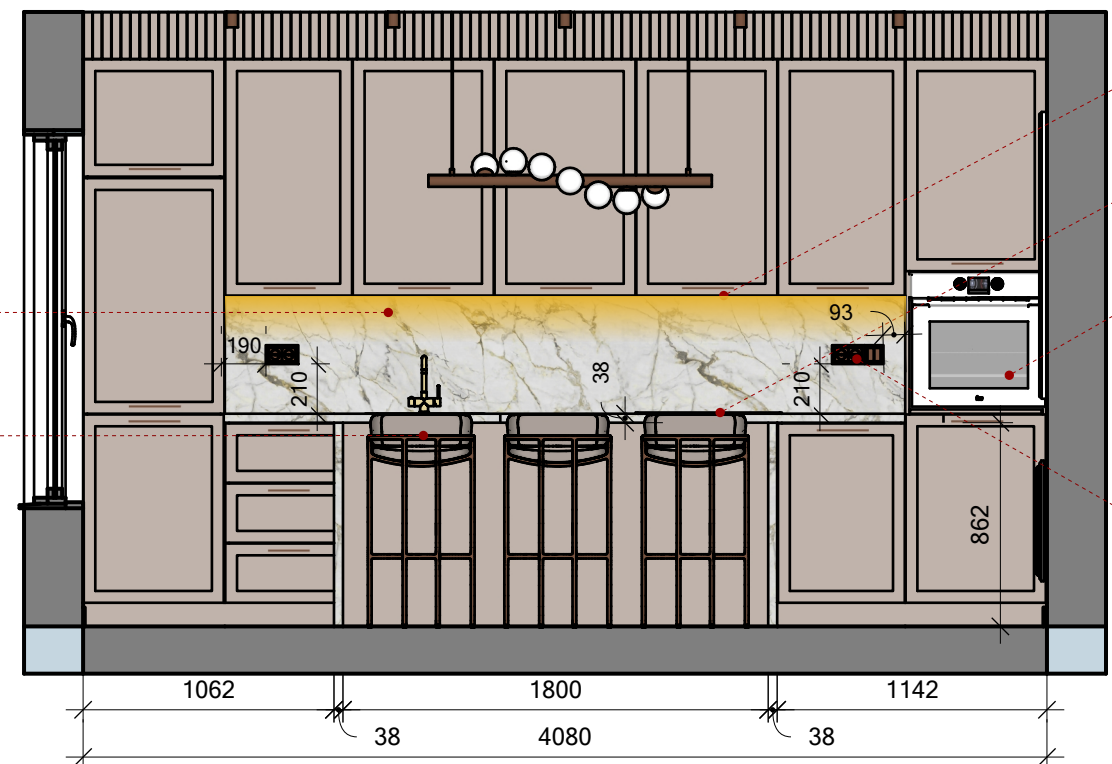
Kuhinja-šank i fronte B 002 M 1:32
